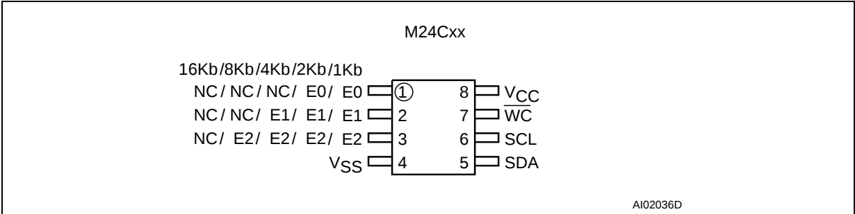
Figure 2C. TSSOP Connections
