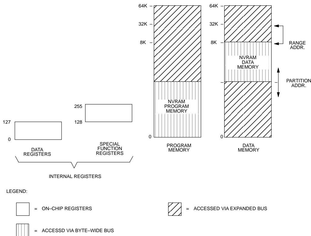
MEMORY MAP OF THE DS5000FP Figure 2
