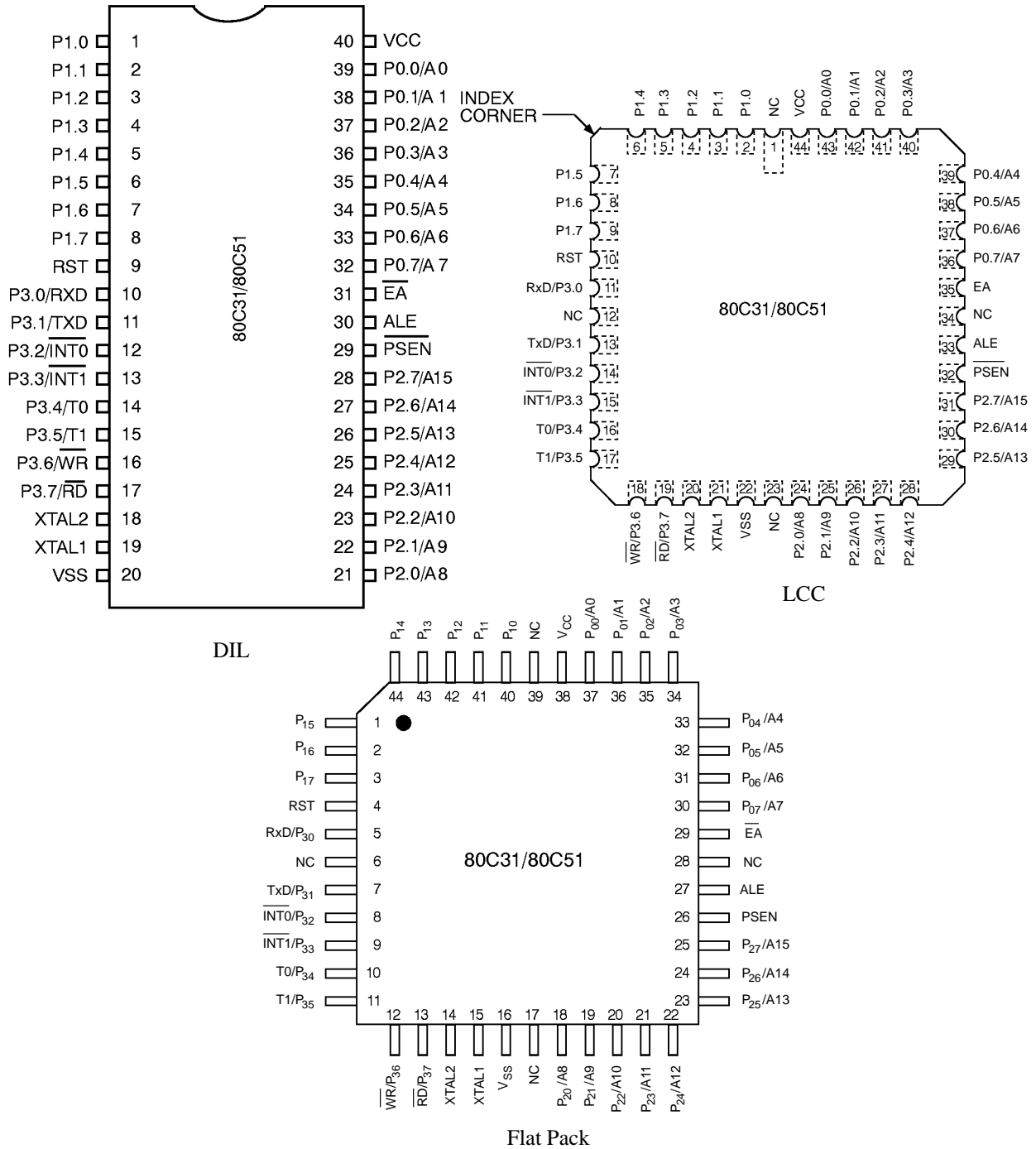
Figure 2. Pin Configuration
