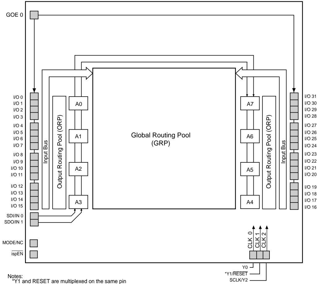
Figure 1. ispLSI 2032 Functional Block Diagram
