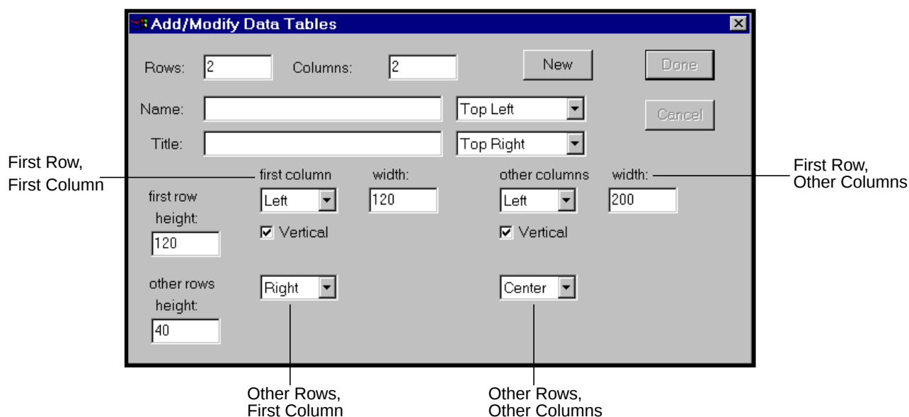
Figure 5. Add/Modify Data Tables Dialog Box
