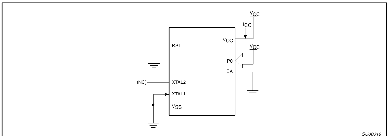
Figure 11. I CC Test Condition, Power Down Mode All other pins are disconnected. V CC = 2V to 5.5V
