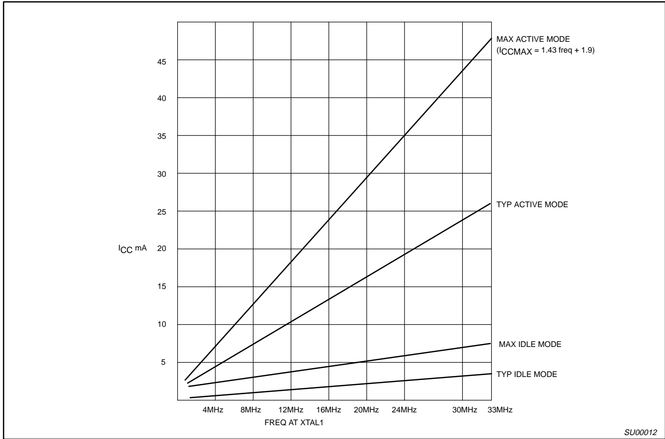
Figure 7. I CC vs. FREQ Valid only within frequency specifications of the device under test
