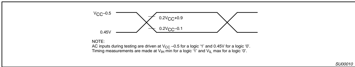
Figure 5. AC Testing Input/Output
