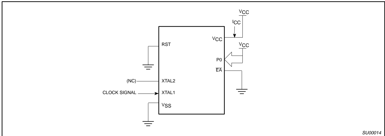
Figure 9. I CC Test Condition, Idle Mode All other pins are disconnected
