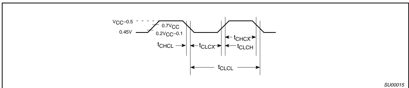
Figure 10. Clock Signal Waveform for I CC Tests in Active and Idle Modes t_{CLCH} = t_{CHCL} = 5\text{ns}
