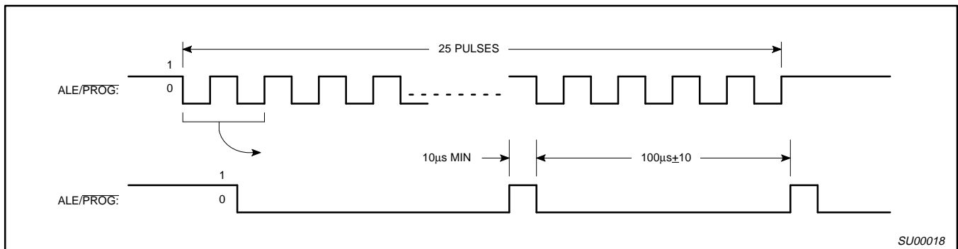
Figure 13. PROG Waveform
