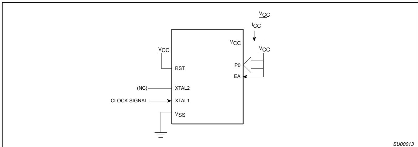
Figure 8. I CC Test Condition, Active Mode All other pins are disconnected
